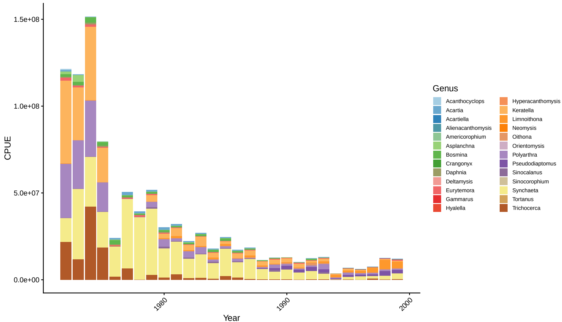
Stacked CPUE by Genus
